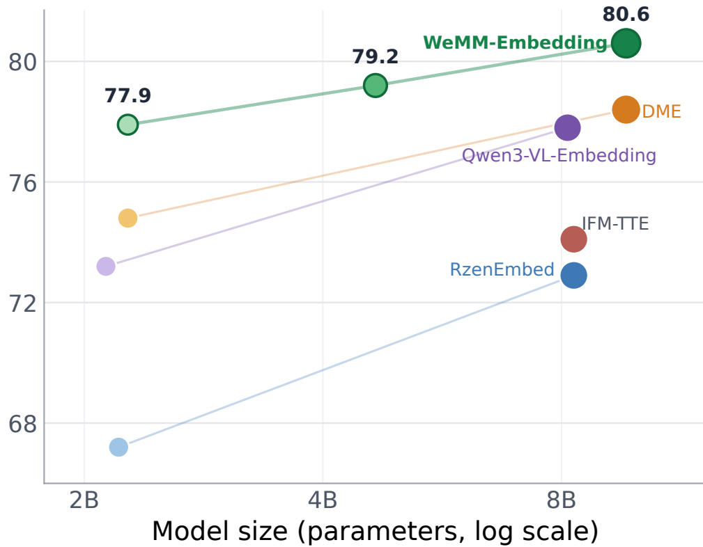
MMEB-v2 Performance
